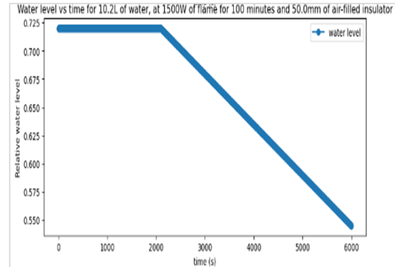
Water Level vs. Time Graph (50mm Insulator)
