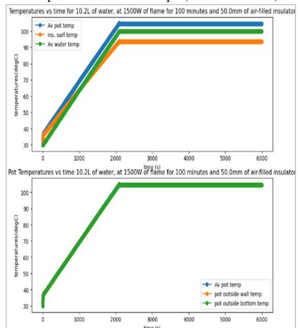
Temperature vs. Time Graph (50mm Insulator)
