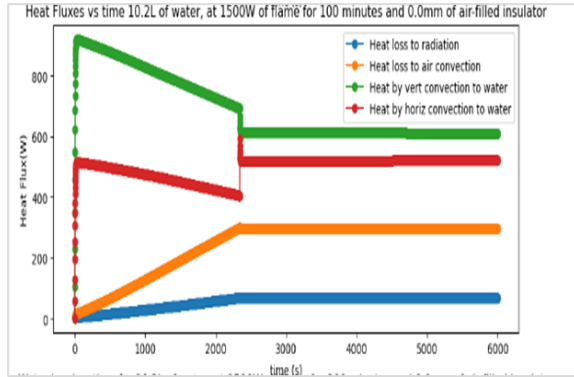
Heat Fluxes vs. Time Graph (0mm Insulator)
