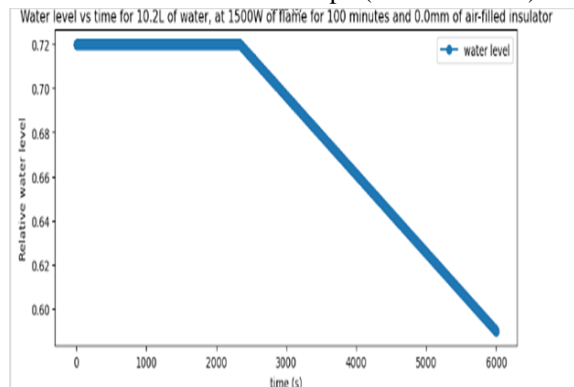
Water Level vs. Time Graph (0mm Insulator)
