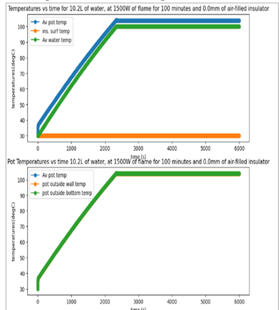
Temperature vs. Time Graph (0mm Insulator)
