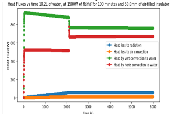
Heat Fluxes vs. Time Graph (50mm Insulator)
