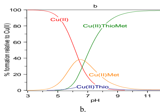
Figure 2: Distribution of species of Metal complexes with pH at 35 °C
