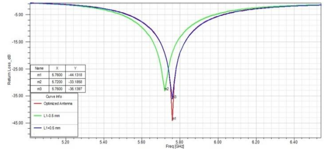
Fig.3 Return loss plot for base shape and L-shaped & DGS
