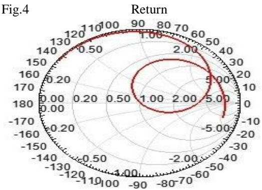
Fig.5 Smith chart of L-shaped patch antenna
